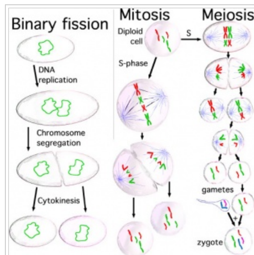
Cell division - 3 types
